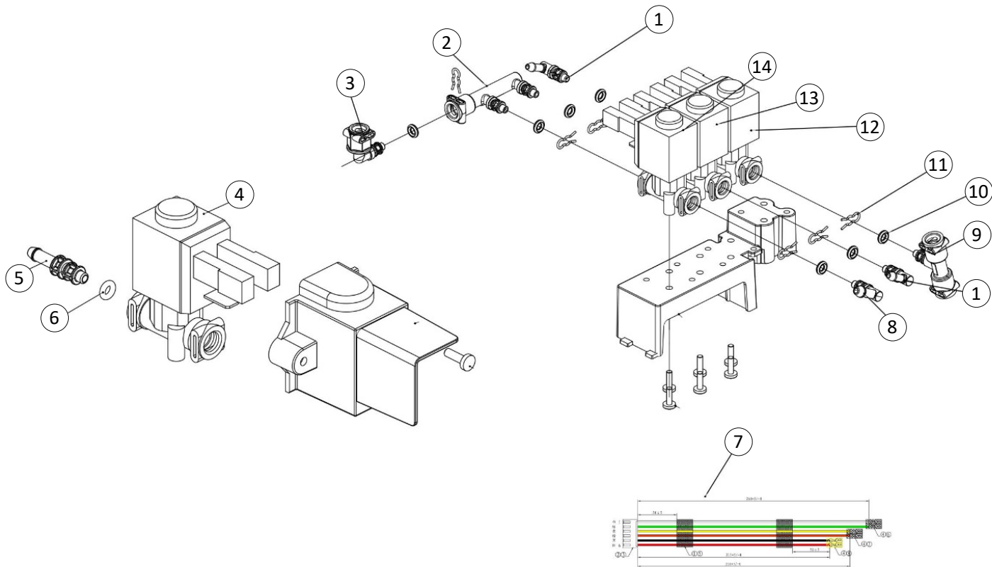
Solenoid valve 1P –hot water
