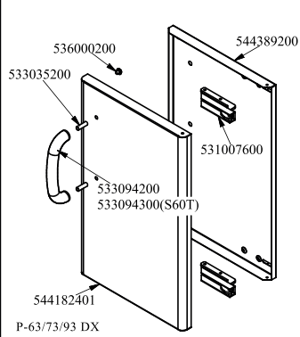
P-63/73/93 DX
