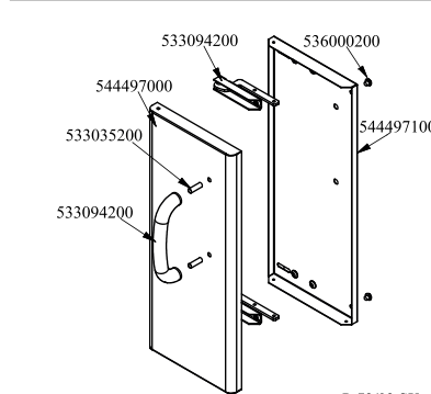
P-72/92 SX
